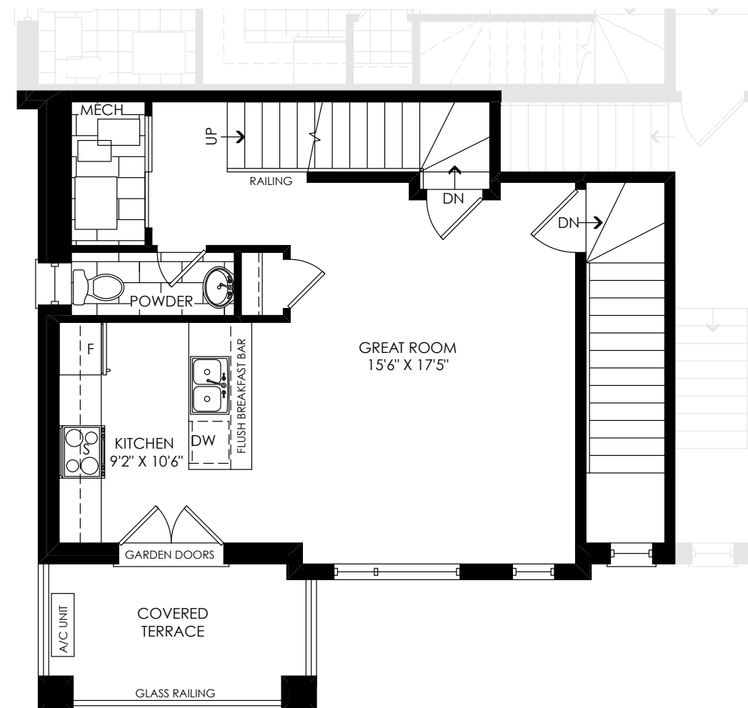
EXTERIOR UPGRADE SECOND FLOOR PLAN (FRONT)
