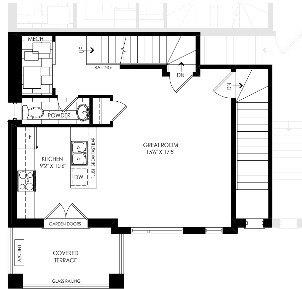
INTERIOR END SECOND FLOOR PLAN (FRONT)
