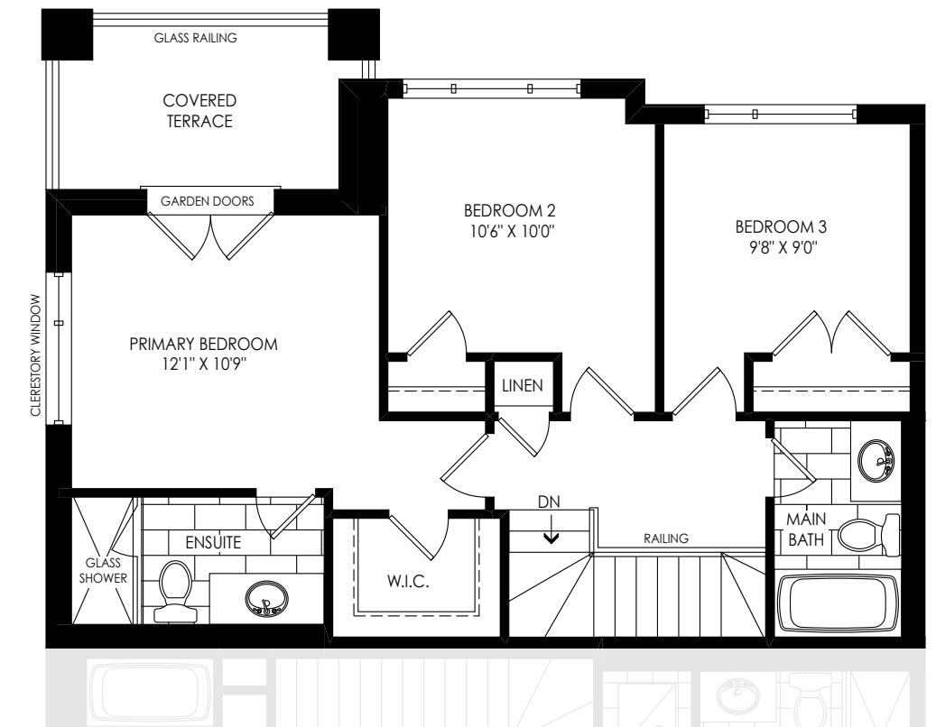
INTERIOR END THIRD FLOOR PLAN (REAR)
